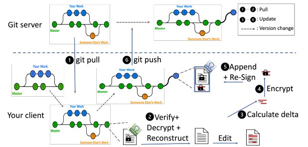
Figure 5: The main workflow of SGitChar
