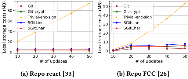
Figure 11: Storage costs of repositories using different schemes.
